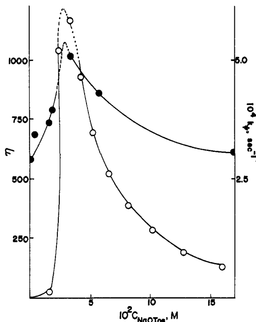
Figure 5. Comparison of the effect of NaOTos on the catalysis by CTABr and on CTABr solution viscosity at 25°C: (○) viscosity for 2.5 \times 10^{-2} M CTABr; (●) k_p in 1.9 \times 10^{-2} M CTABr.
