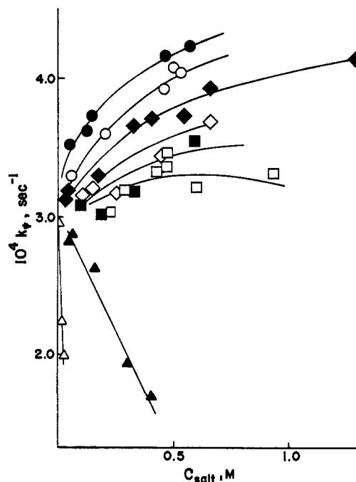
Figure 3. The effect of salts on the catalysis by 2 \times 10^{-2} M CTABr in 0.002 M NH 3 buffer, 25^\circ : (●) Na 2 SO 4 ; (○) NaBr; (◆) MCl ( M = \text{Li, Na, Me}_4\text{N} ); (◇) NaF; (■) NaOAc; (□) NaOH; (▲) sodium pivalate; (△) NaCNS.
