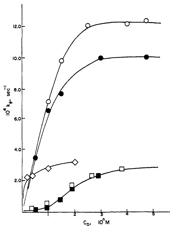
Figure 1. Micellar catalysis of the decarboxylation of 6-nitrobenzisoxazole-3-carboxylate at 25.0°: (□) CTABr in 0.002 M NaOH, n = 3; (■) CTABr in 0.002 M NH 3 buffer (pH 9), n = 3; (◇) N -cetylpyridinium bromide in 0.002 M NH 3 buffer, n = 2; dicationic surfactants IIb (●) and IIc (○) in 0.002 M NH 3 , n = 4.
